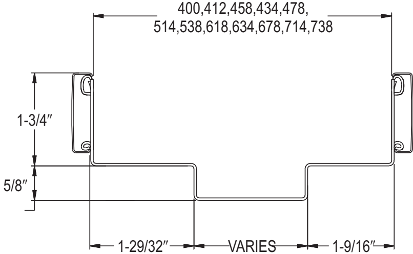
REDIFRAME SECTION NO GLAZING BEAD
