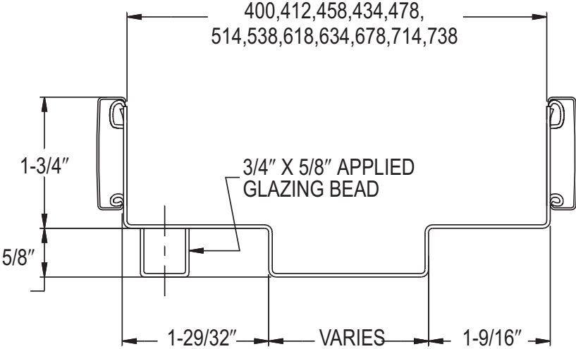
REDIFRAME SECTION WITH APPLIED GLAZING BEAD
