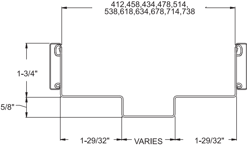
1-3/4" x 1-3/4" COMMUNICATING FRAME
