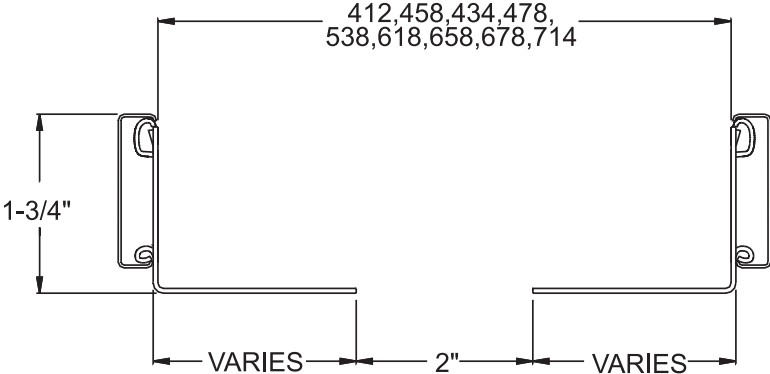
POCKET DOOR FRAME 1-3/4" DOOR ONLY
