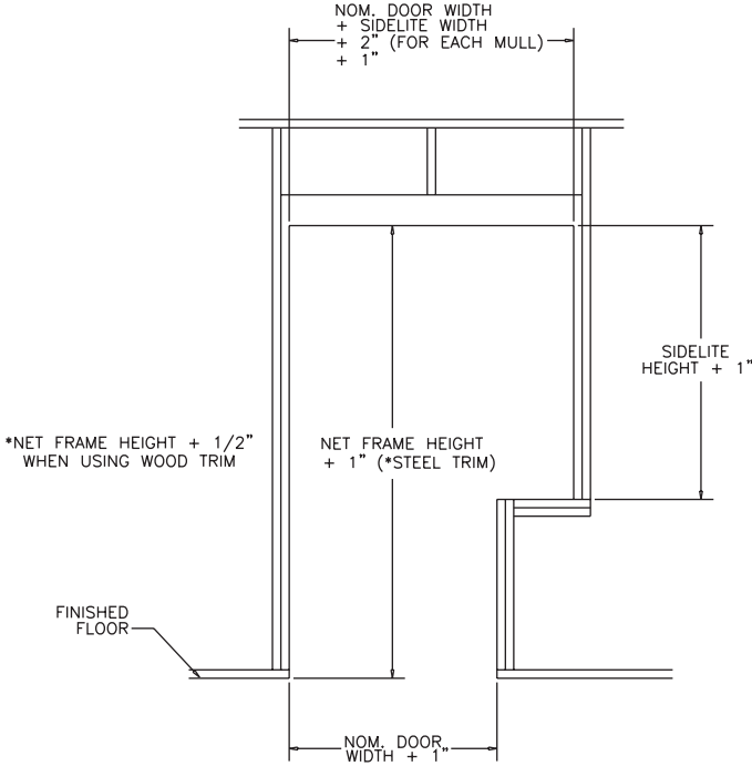
PARTIAL SIDELITE ROUGH OPENING
