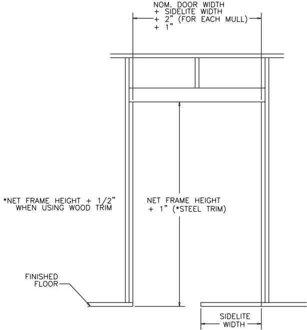
STANDARD SIDELITE ROUGH OPENING
